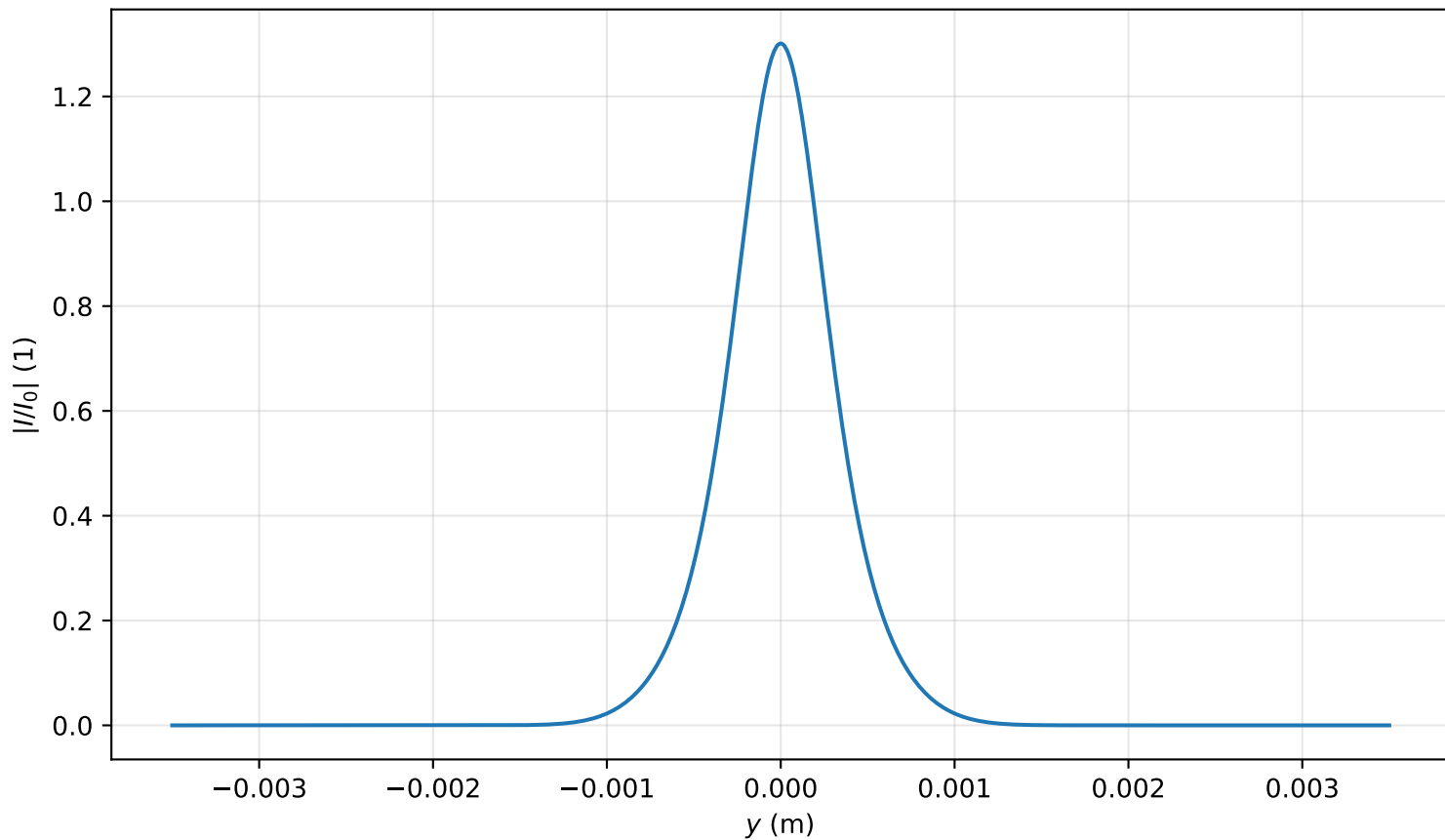
Intensity profile I(x=0, y, z=0.796)/I_0 , P_{in}=0.9P_{cr} , artificial time
